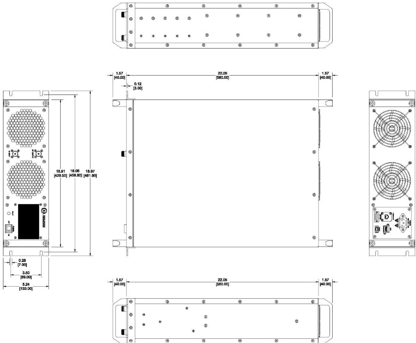
OUTLINE DRAWING-3U Shown with optional LCD
